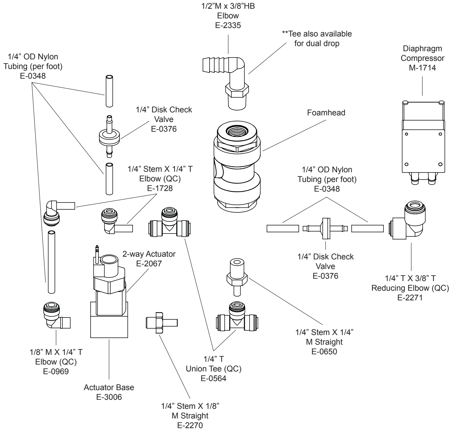
FIGURE 3 - TurfMarker 2010 Power Unit Internal Components
