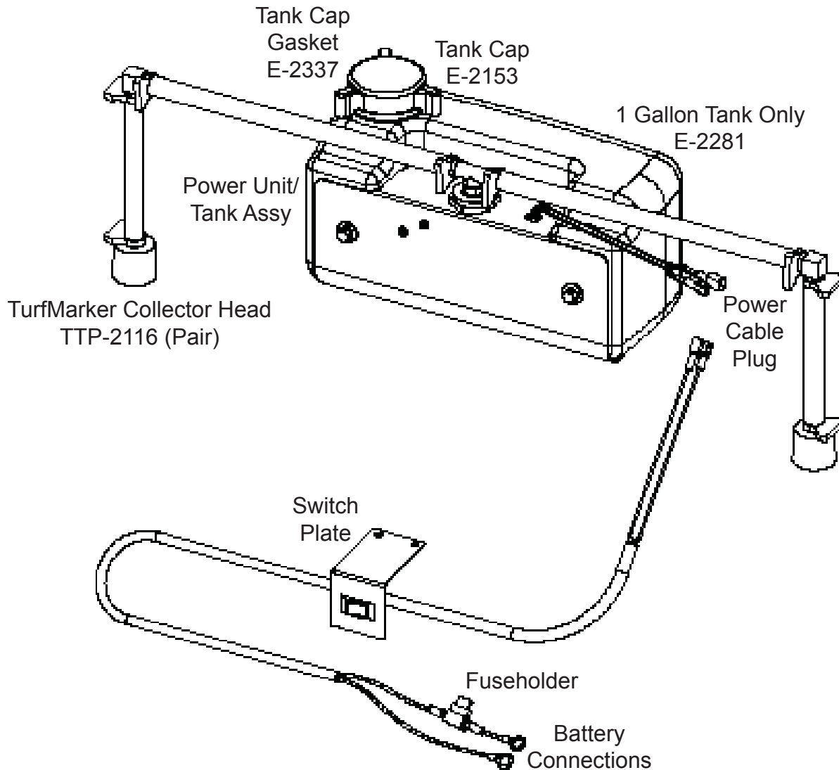
FIGURE 1 - TurfMarker Model TF-2010 Foam Marker
